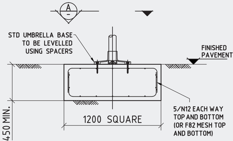
FOOTING OPTION B - PAD FOOTING
