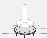
Base Plate 315mm \phi - to bolt to concrete patio or wooden deck
